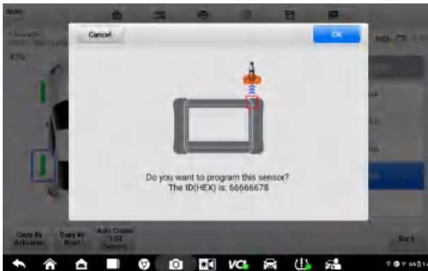
Figure 5-6 Copy by Activation Function Screen
