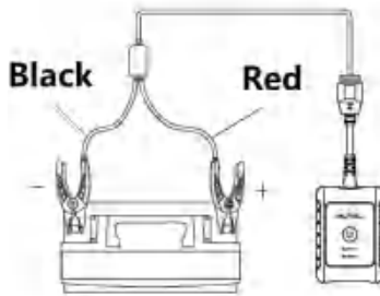
Figure 9-2 Connecting to a Battery
